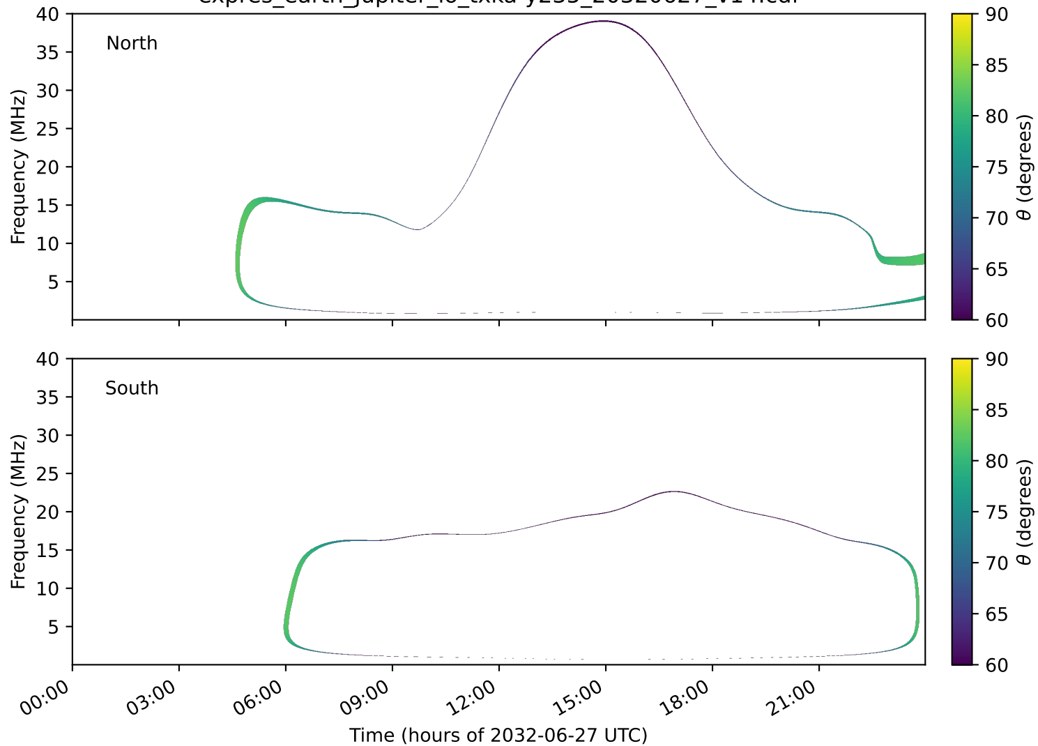
expres_earth_jupiter_io_txka-y235_20320627_v14.cdf
