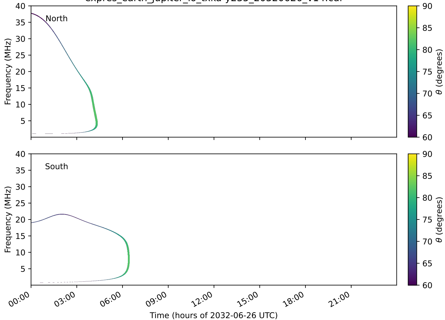
expres_earth_jupiter_io_txka-y235_20320626_v14.cdf
