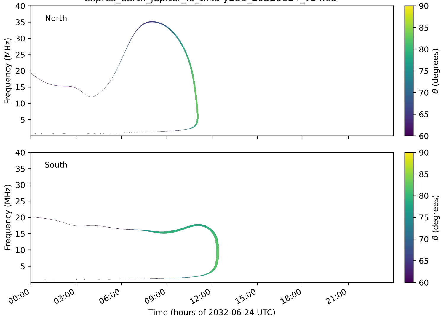
expres_earth_jupiter_io_txka-y235_20320624_v14.cdf
