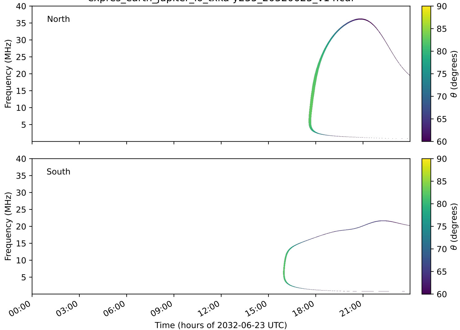
expres_earth_jupiter_io_txka-y235_20320623_v14.cdf
