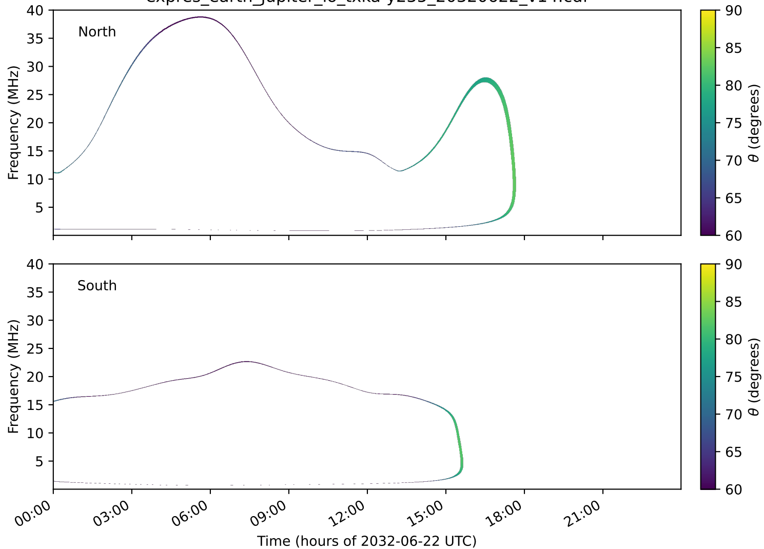
expres_earth_jupiter_io_txka-y235_20320622_v14.cdf
