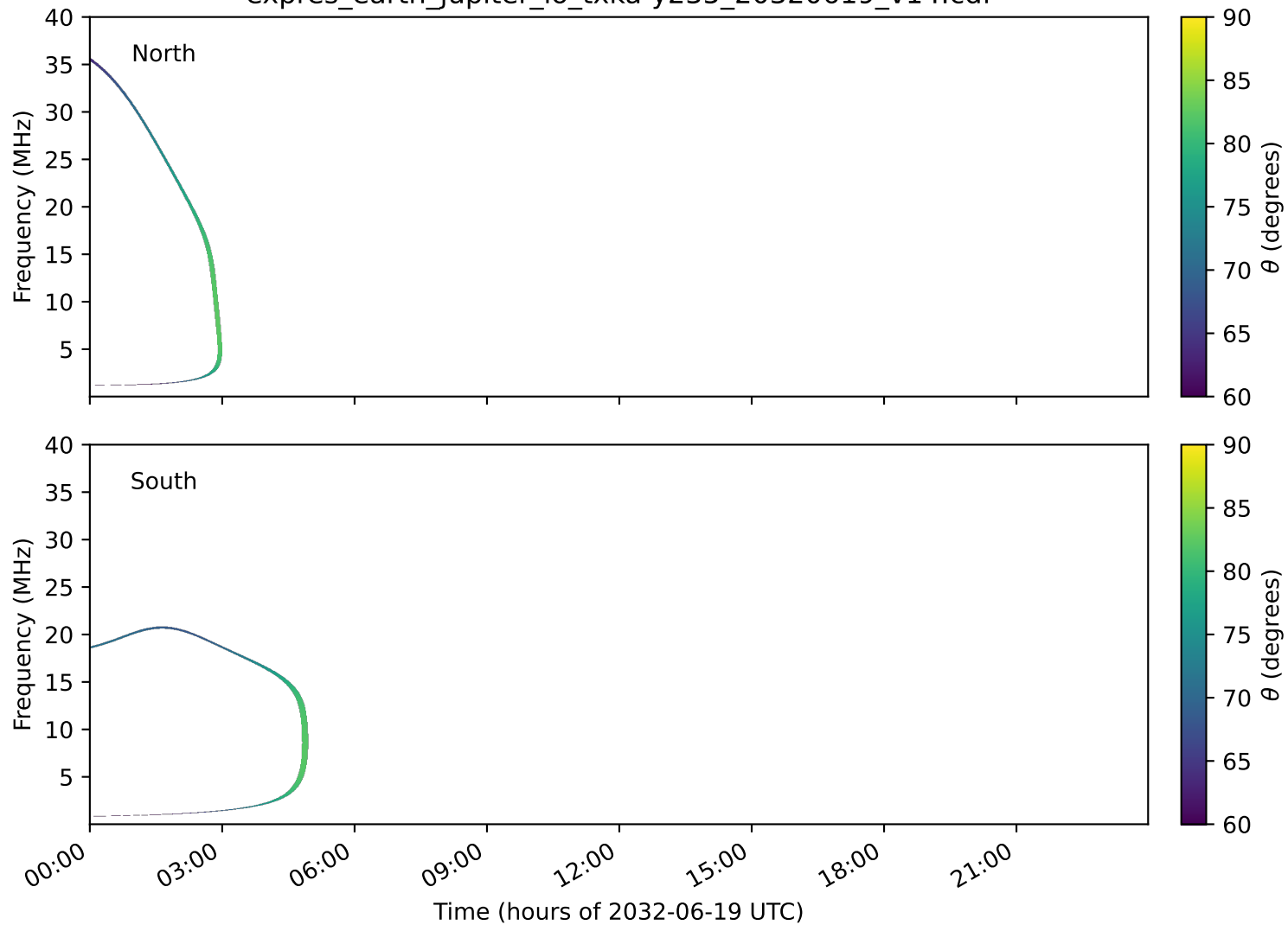
expres_earth_jupiter_io_txka-y235_20320619_v14.cdf
