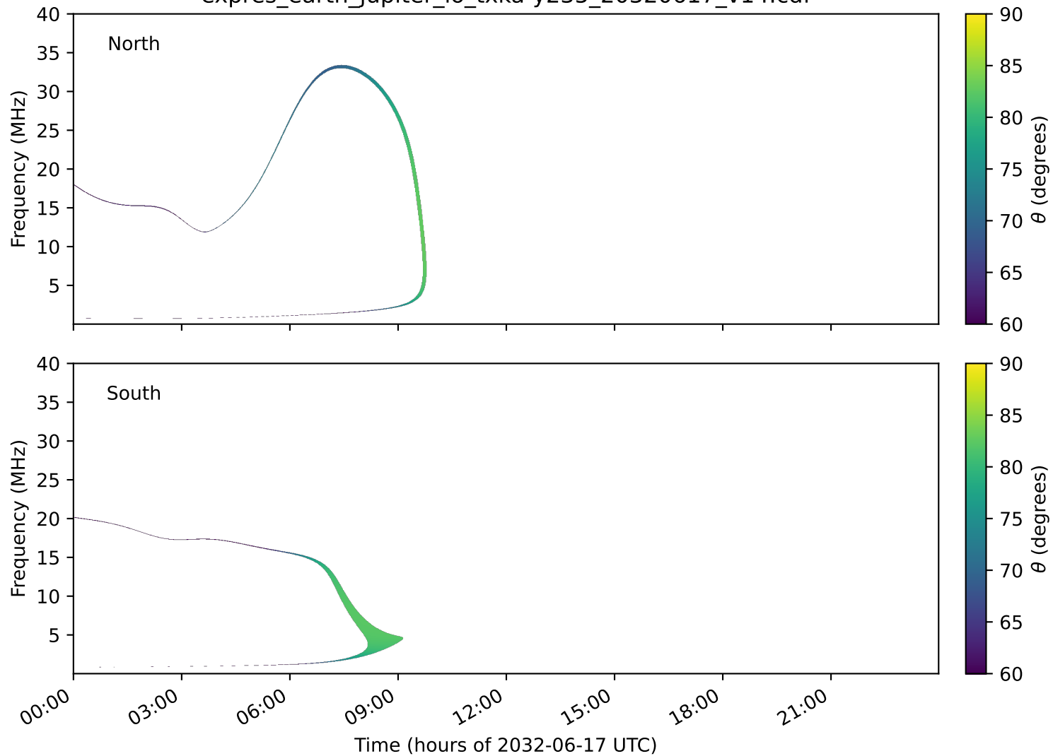
expres_earth_jupiter_io_txka-y235_20320617_v14.cdf
