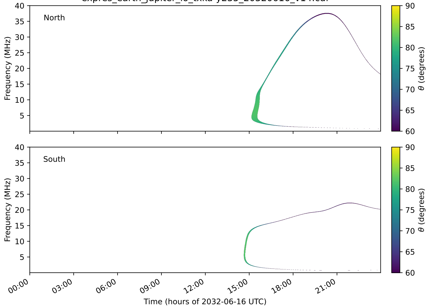
expres_earth_jupiter_io_txka-y235_20320616_v14.cdf
