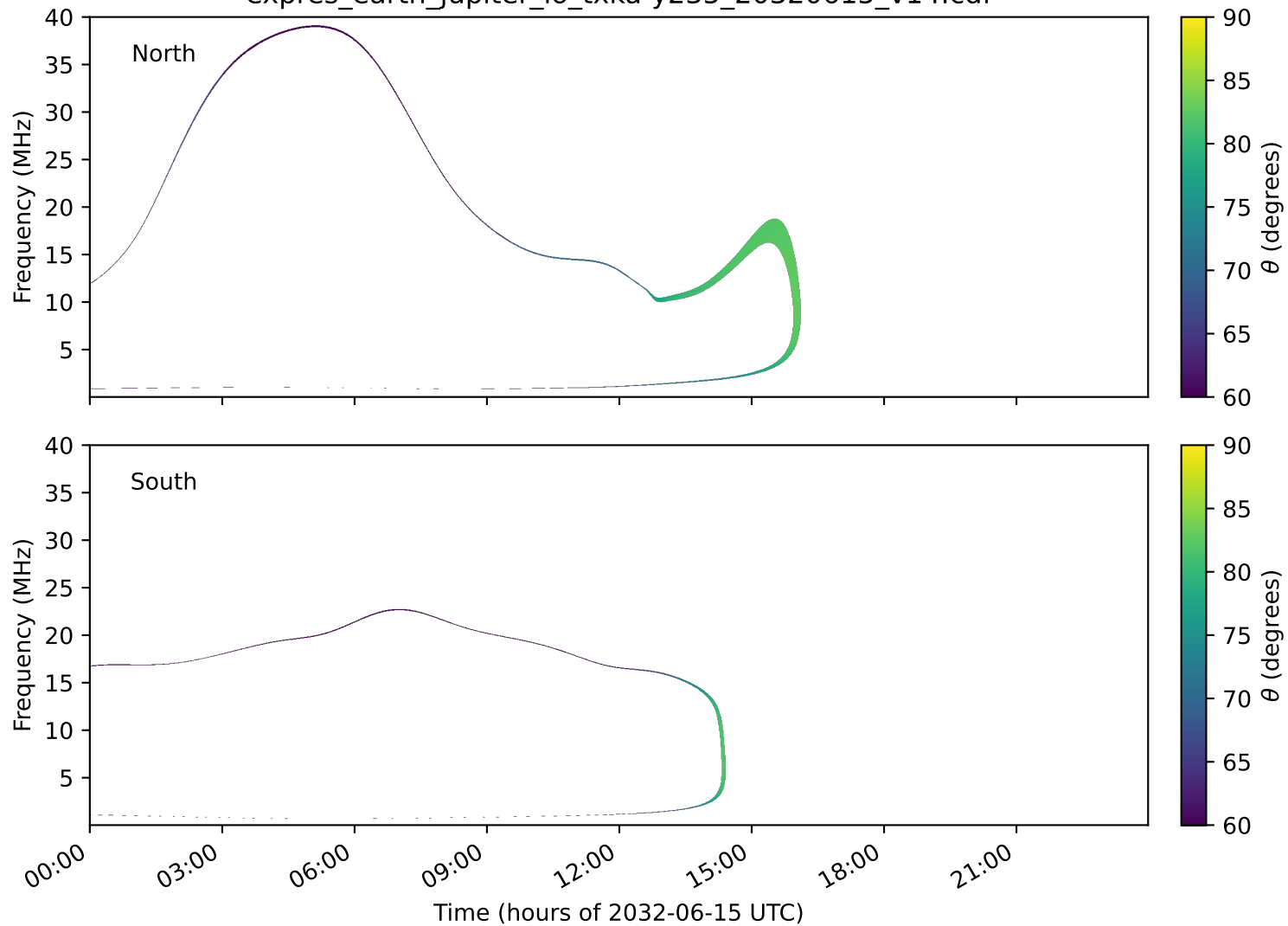
expres_earth_jupiter_io_txka-y235_20320615_v14.cdf
