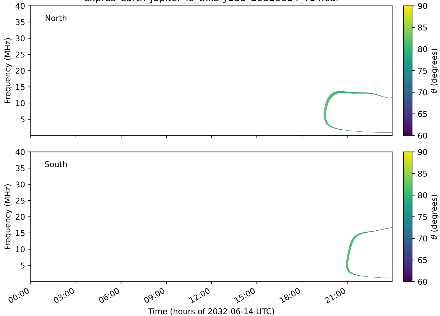
expres_earth_jupiter_io_txka-y235_20320614_v14.cdf
