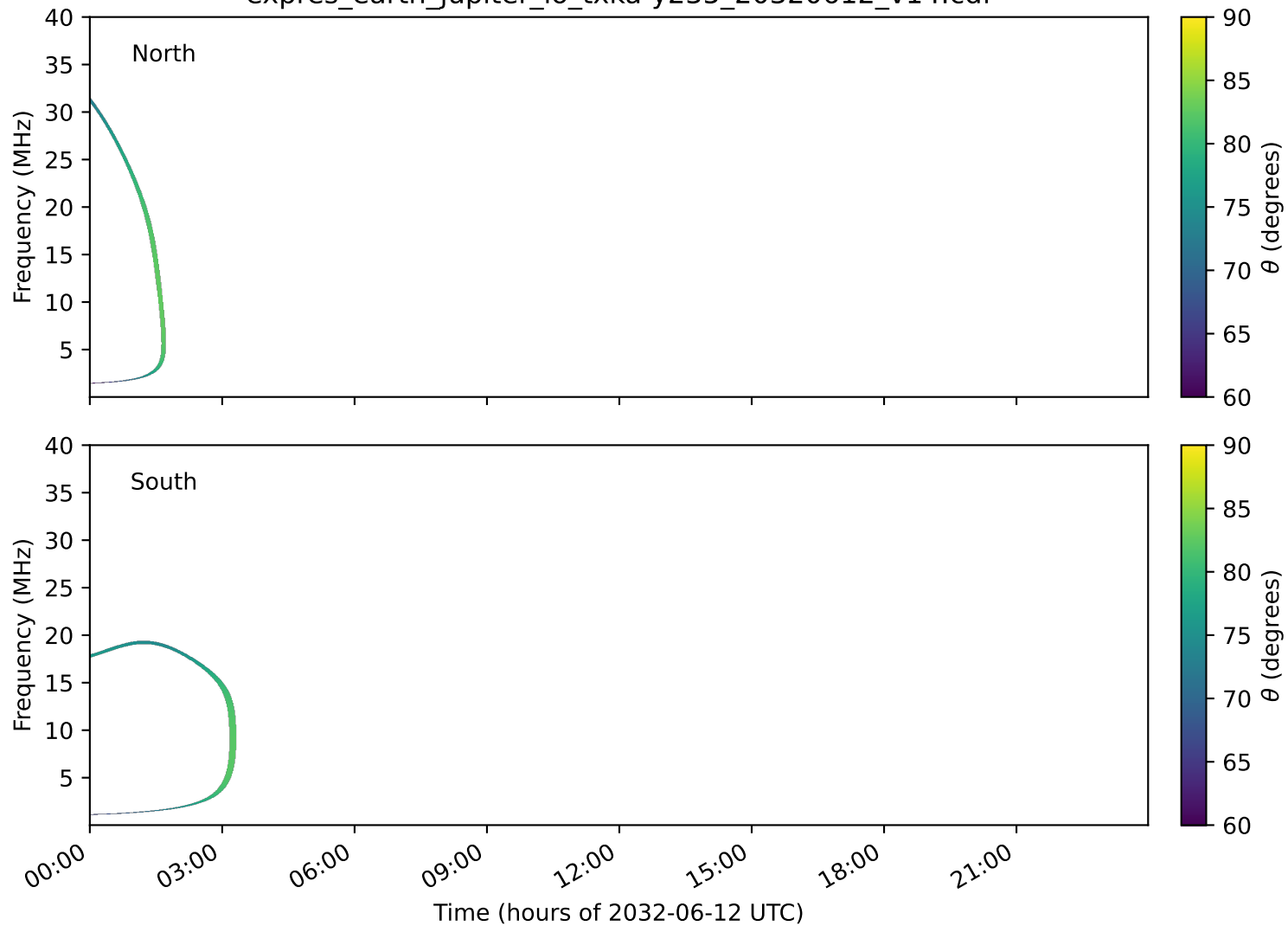
expres_earth_jupiter_io_txka-y235_20320612_v14.cdf
