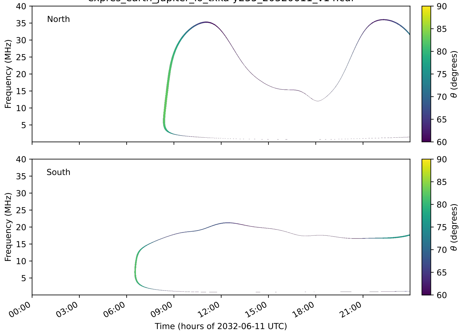
expres_earth_jupiter_io_txka-y235_20320611_v14.cdf
