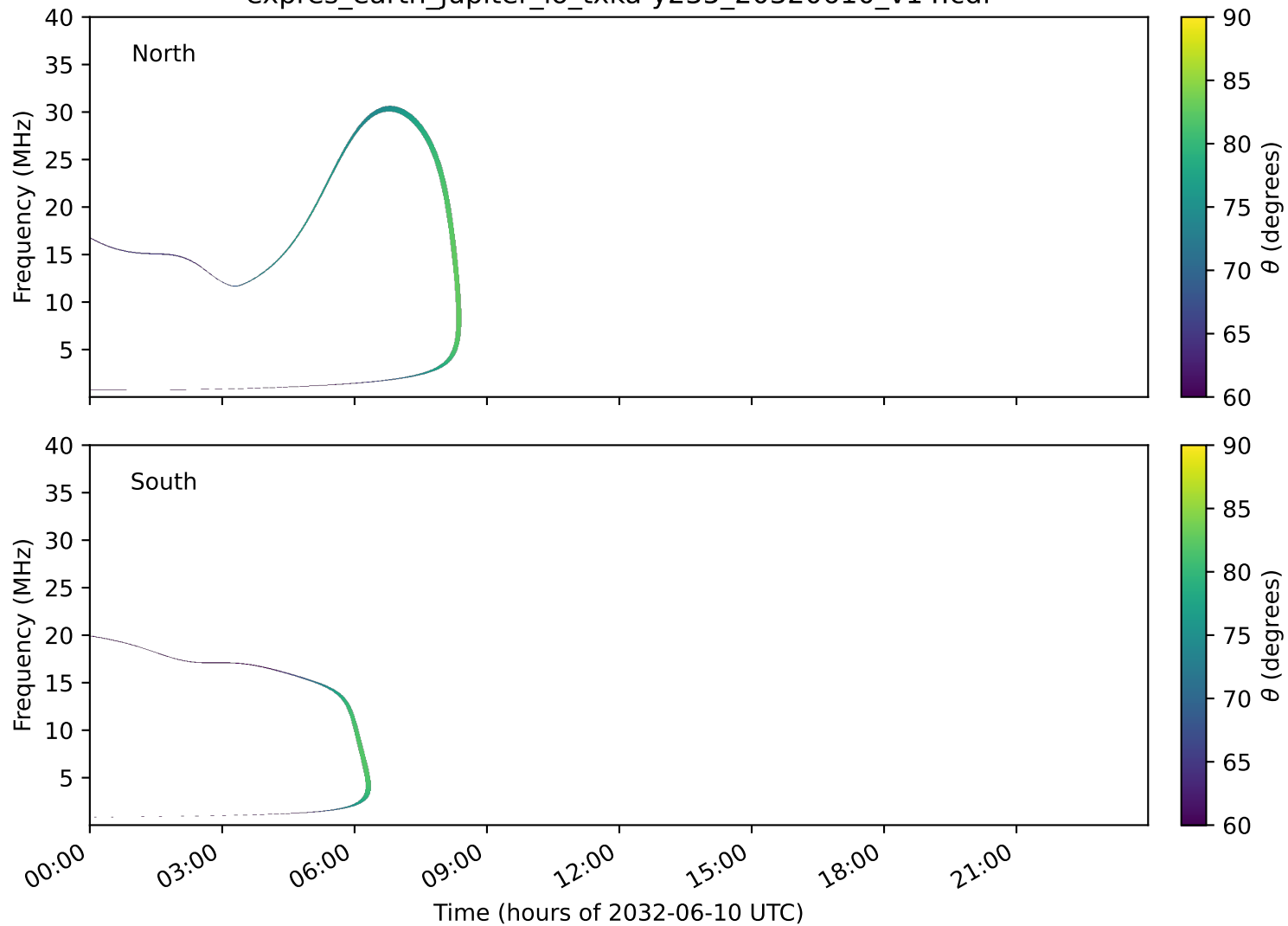
expres_earth_jupiter_io_txka-y235_20320610_v14.cdf
