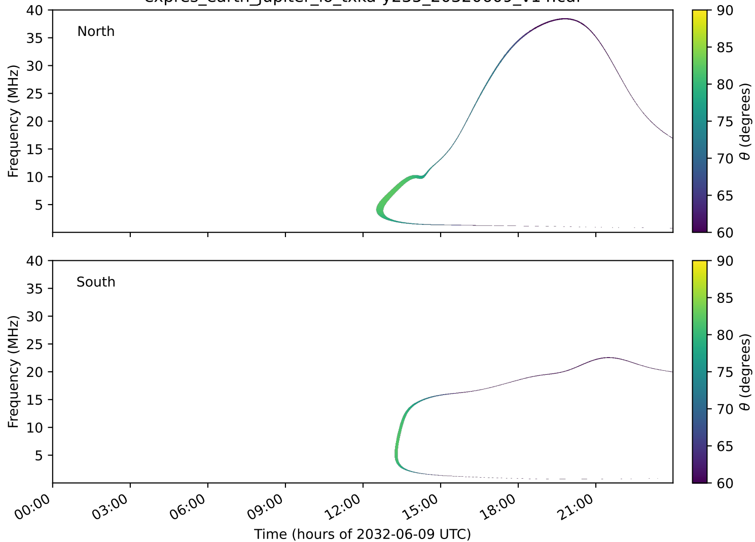
expres_earth_jupiter_io_txka-y235_20320609_v14.cdf
