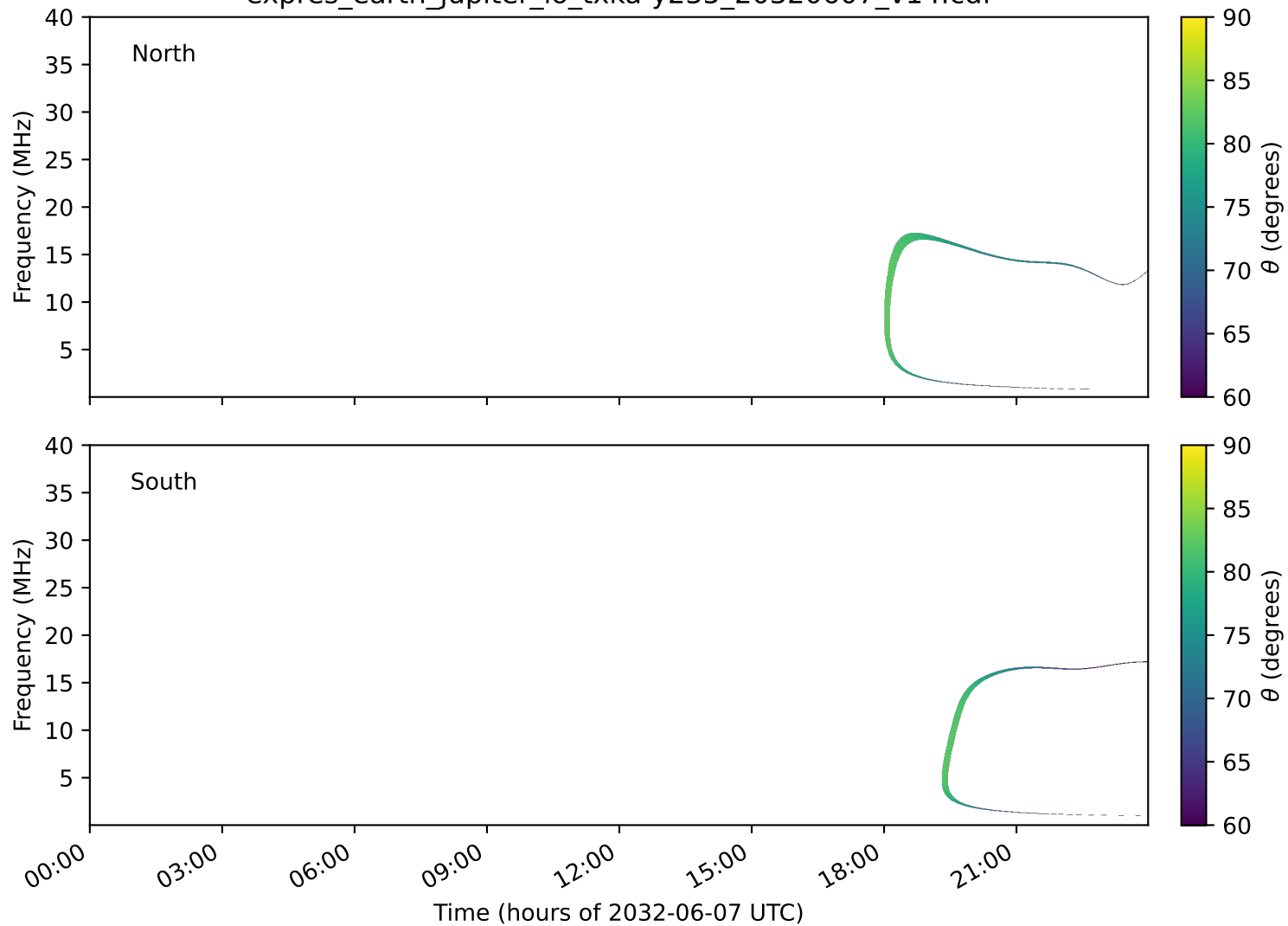
expres_earth_jupiter_io_txka-y235_20320607_v14.cdf
