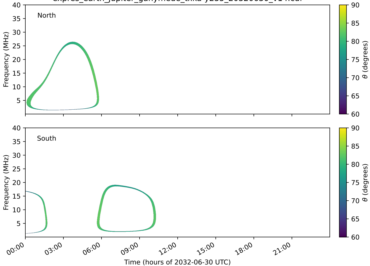
expres_earth_jupiter_ganymede_txka-y235_20320630_v14.cdf
