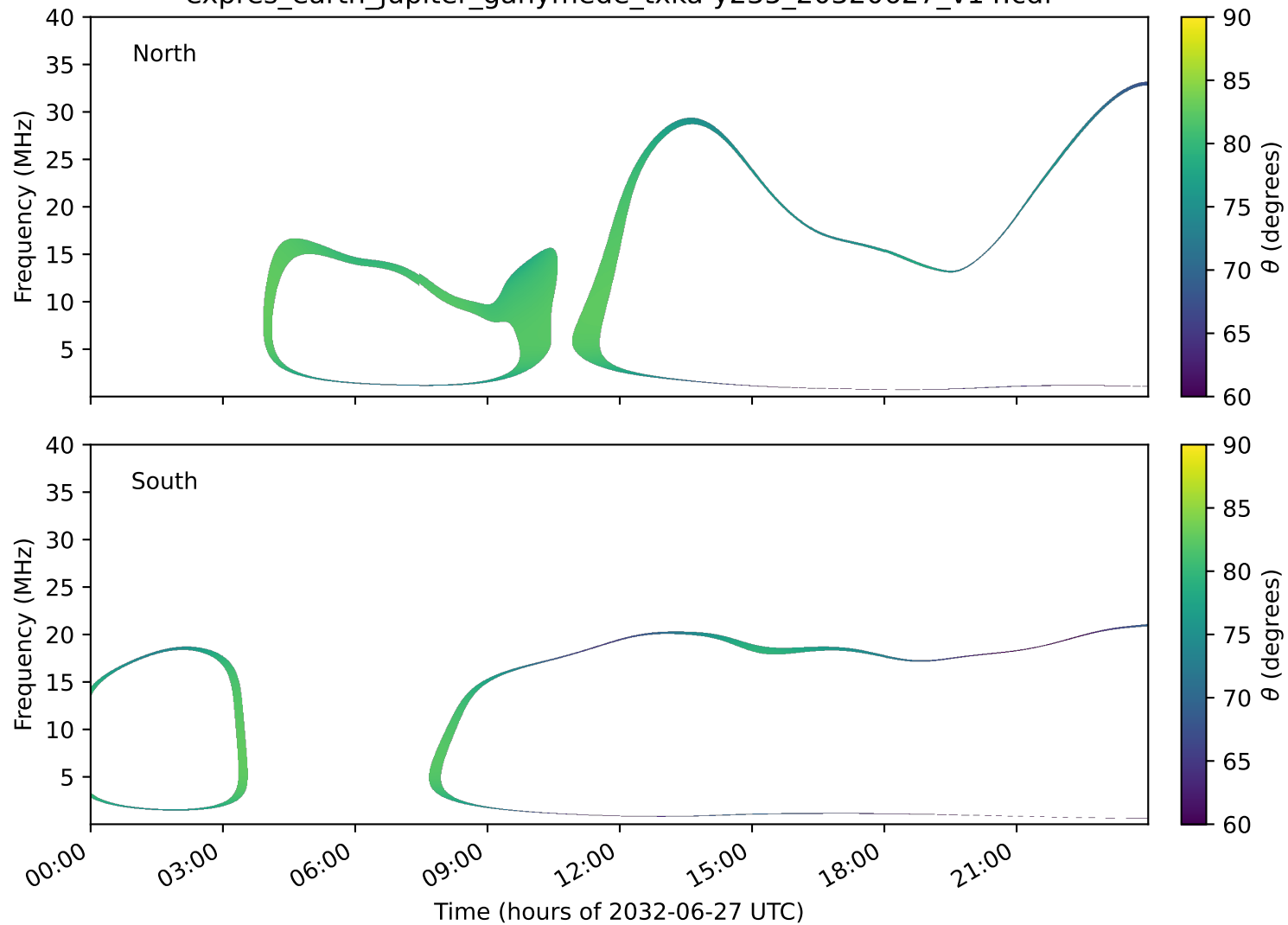
expres_earth_jupiter_ganymede_txka-y235_20320627_v14.cdf
