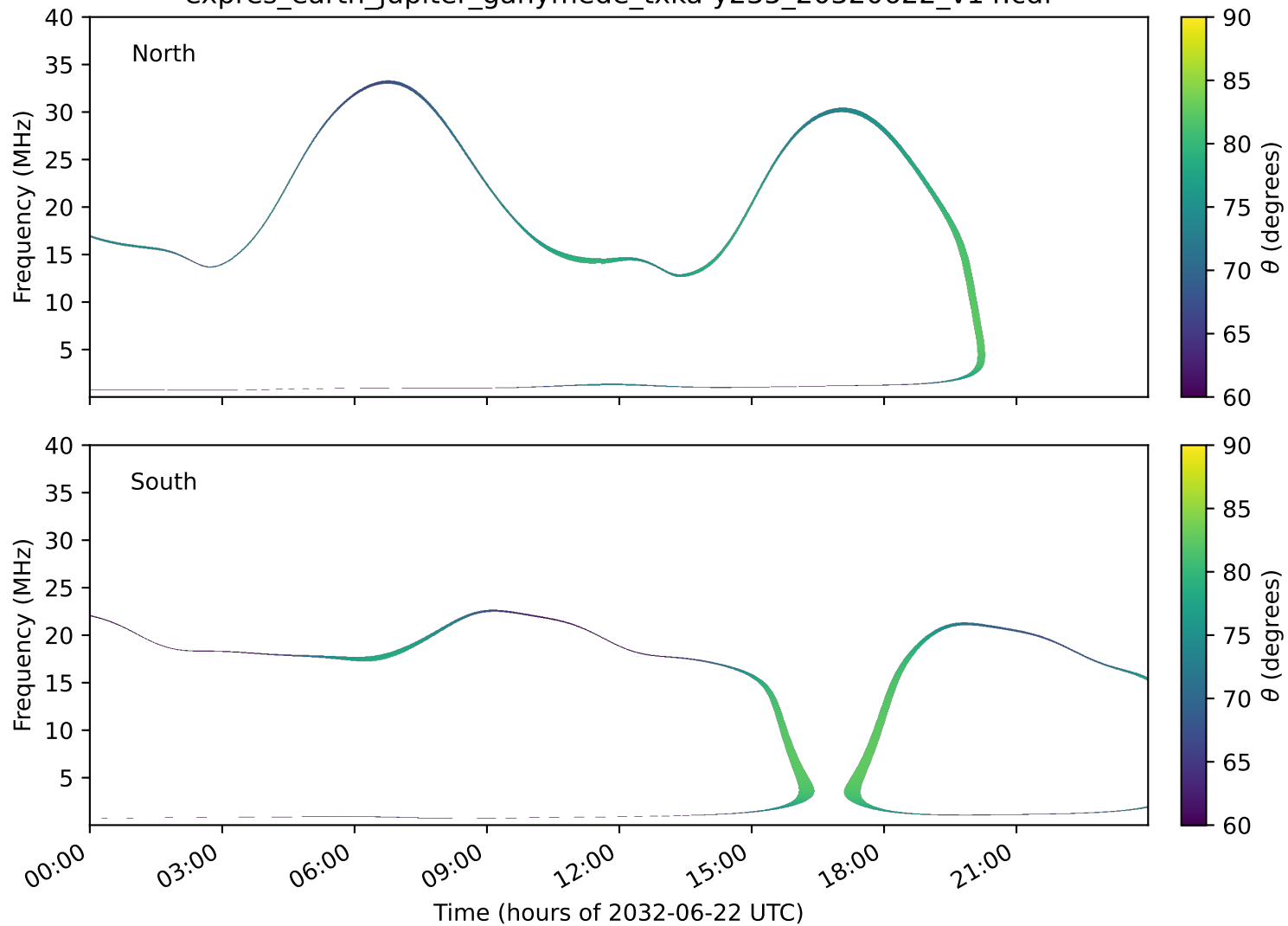
expres_earth_jupiter_ganymede_txka-y235_20320622_v14.cdf
