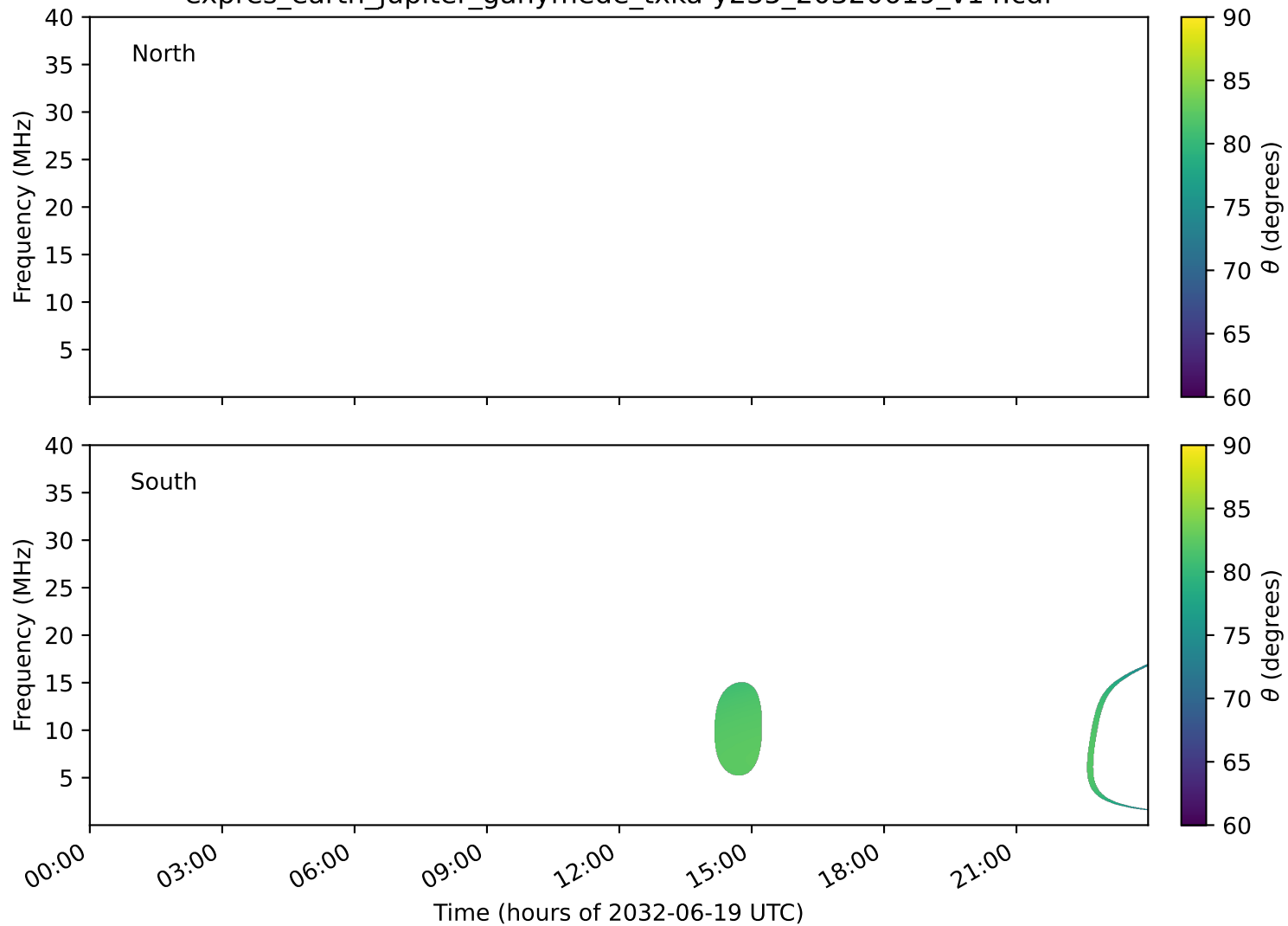
expres_earth_jupiter_ganymede_txka-y235_20320619_v14.cdf
