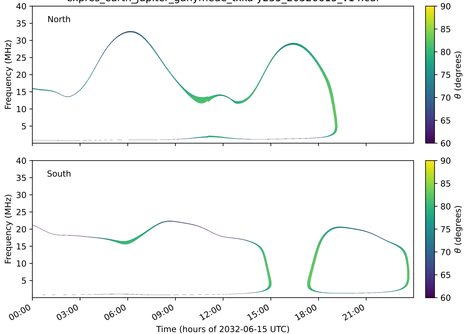
expres_earth_jupiter_ganymede_txka-y235_20320615_v14.cdf
