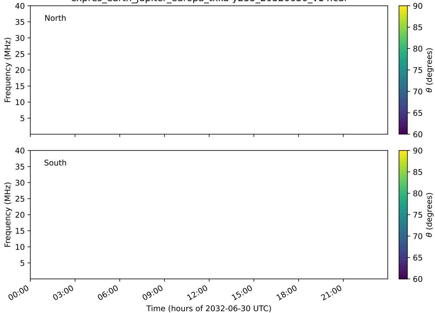
expres_earth_jupiter_europa_txka-y235_20320630_v14.cdf
