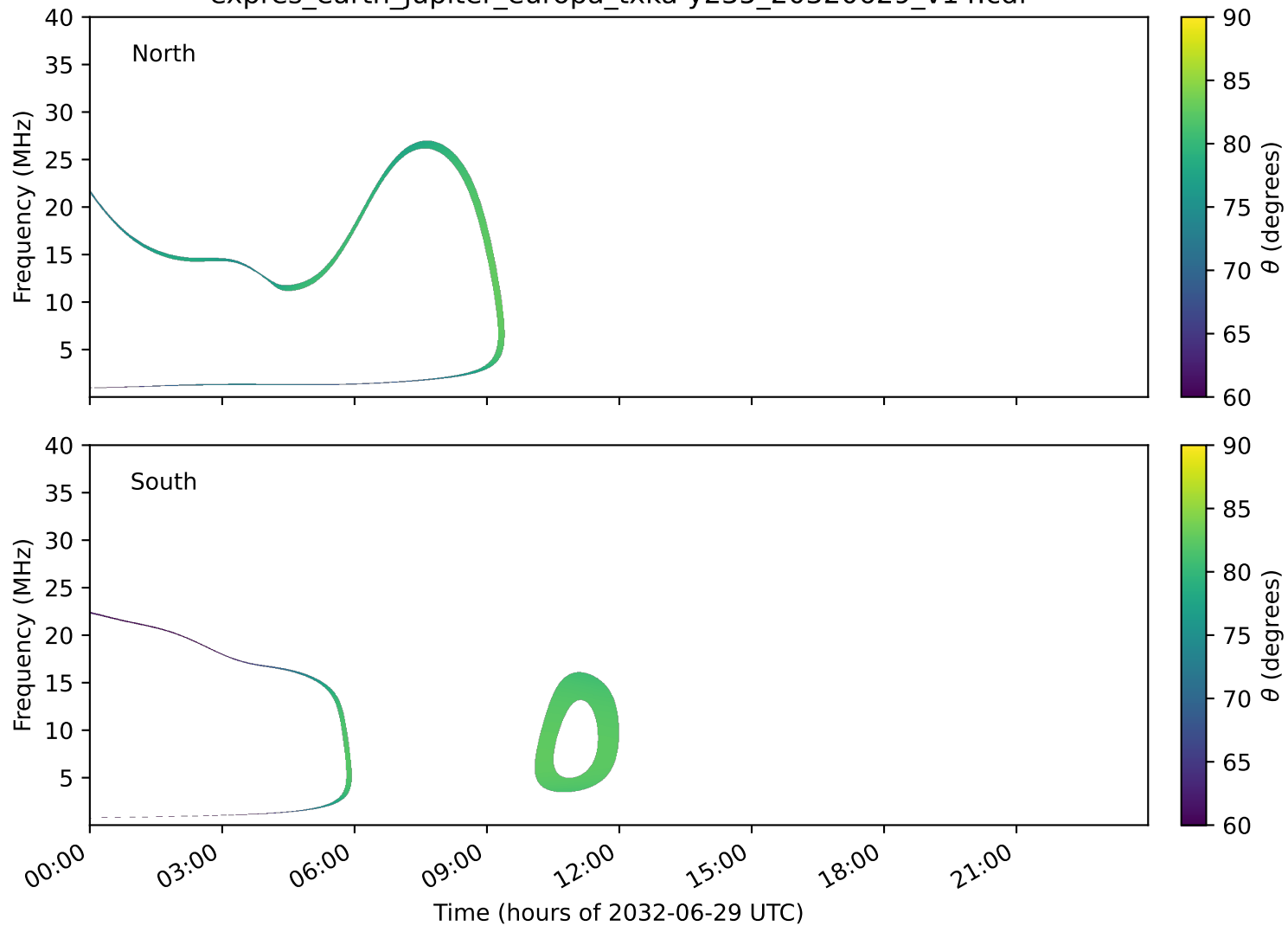
expres_earth_jupiter_europa_txka-y235_20320629_v14.cdf
