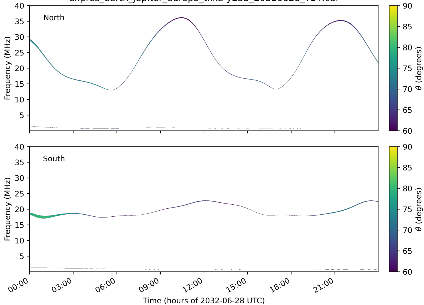
expres_earth_jupiter_europa_txka-y235_20320628_v14.cdf
