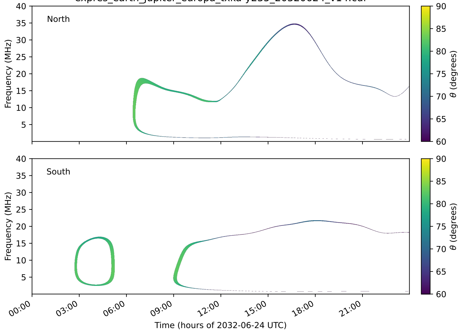
expres_earth_jupiter_europa_txka-y235_20320624_v14.cdf
