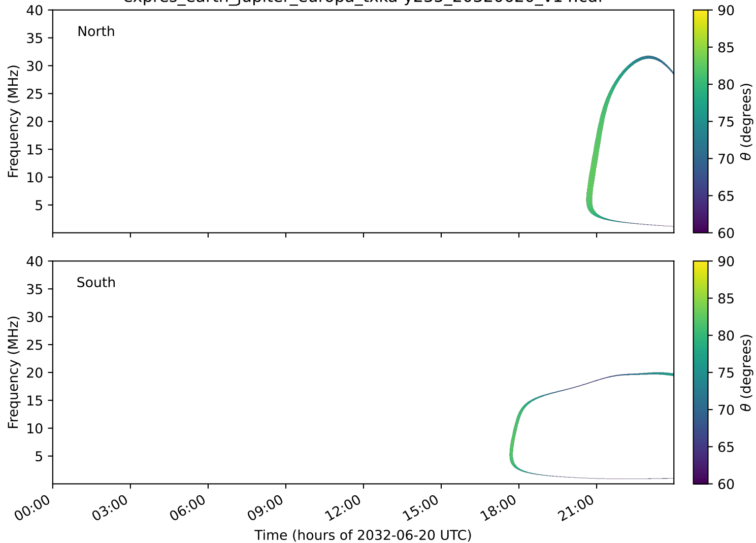
expres_earth_jupiter_europa_txka-y235_20320620_v14.cdf
