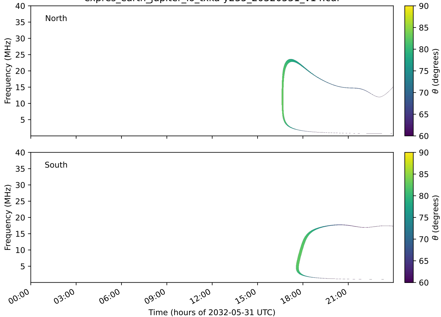
expres_earth_jupiter_io_txka-y235_20320531_v14.cdf
