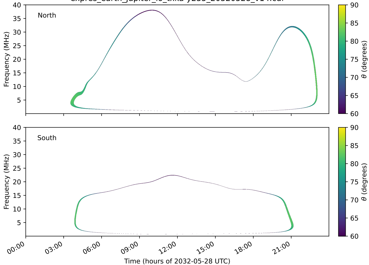
expres_earth_jupiter_io_txka-y235_20320528_v14.cdf
