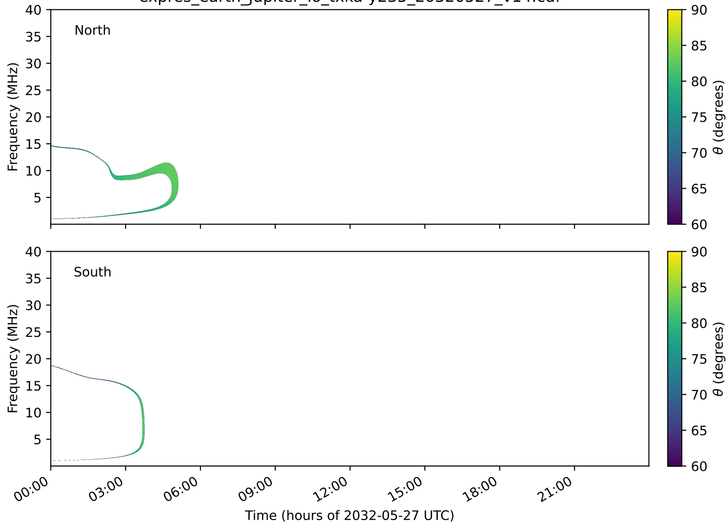
expres_earth_jupiter_io_txka-y235_20320527_v14.cdf
