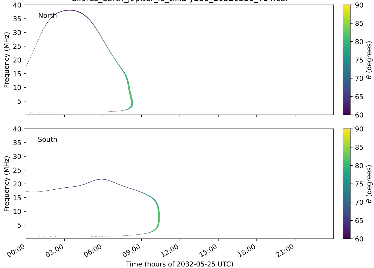
expres_earth_jupiter_io_txka-y235_20320525_v14.cdf
