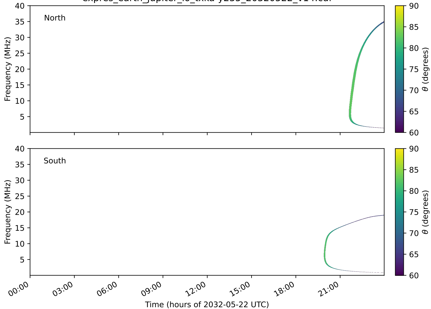
expres_earth_jupiter_io_txka-y235_20320522_v14.cdf
