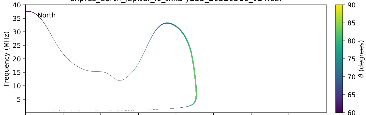
expres_earth_jupiter_io_txka-y235_20320516_v14.cdf
