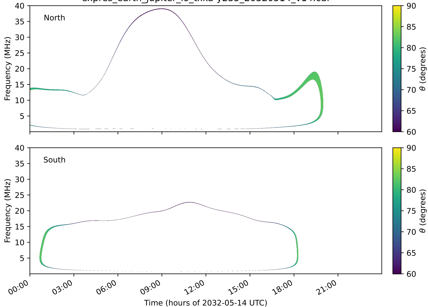
expres_earth_jupiter_io_txka-y235_20320514_v14.cdf
