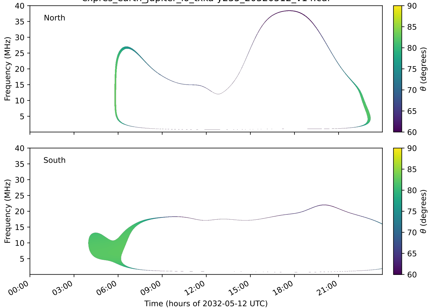
expres_earth_jupiter_io_txka-y235_20320512_v14.cdf
