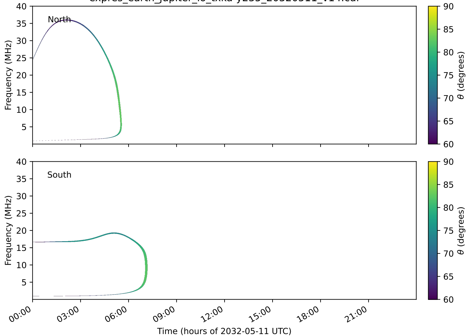
expres_earth_jupiter_io_txka-y235_20320511_v14.cdf
