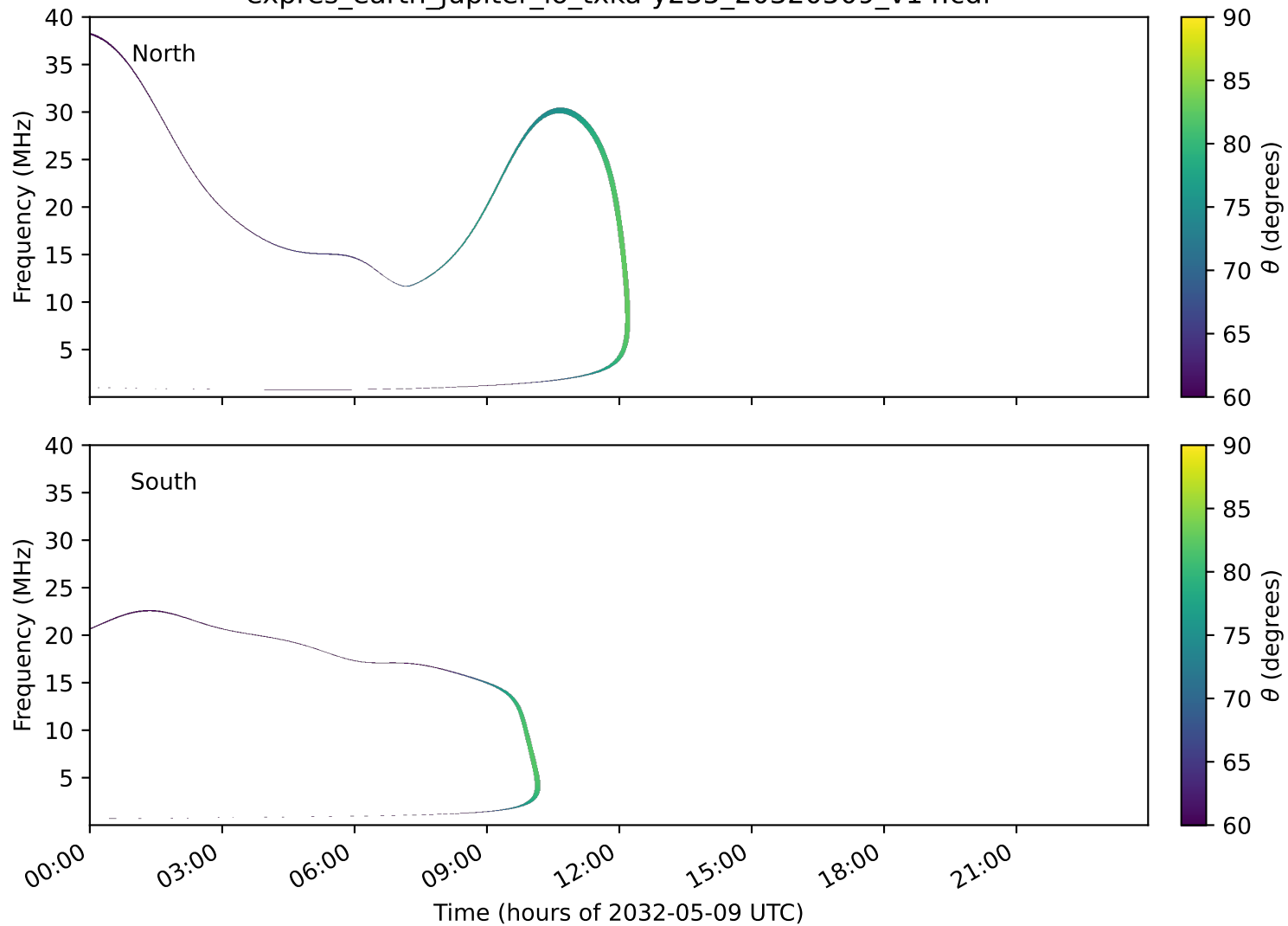
expres_earth_jupiter_io_txka-y235_20320509_v14.cdf
