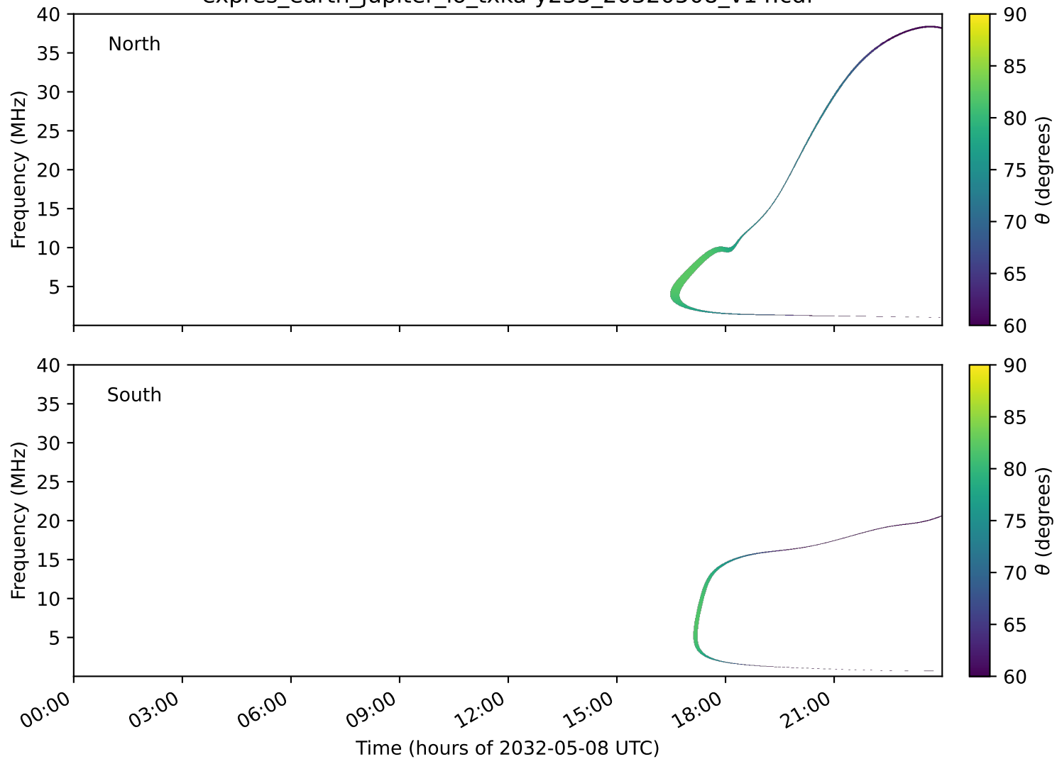
expres_earth_jupiter_io_txka-y235_20320508_v14.cdf
