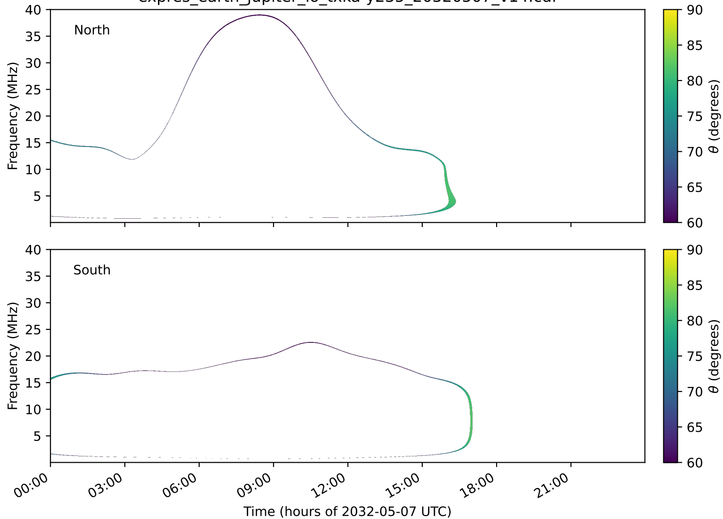
expres_earth_jupiter_io_txka-y235_20320507_v14.cdf
