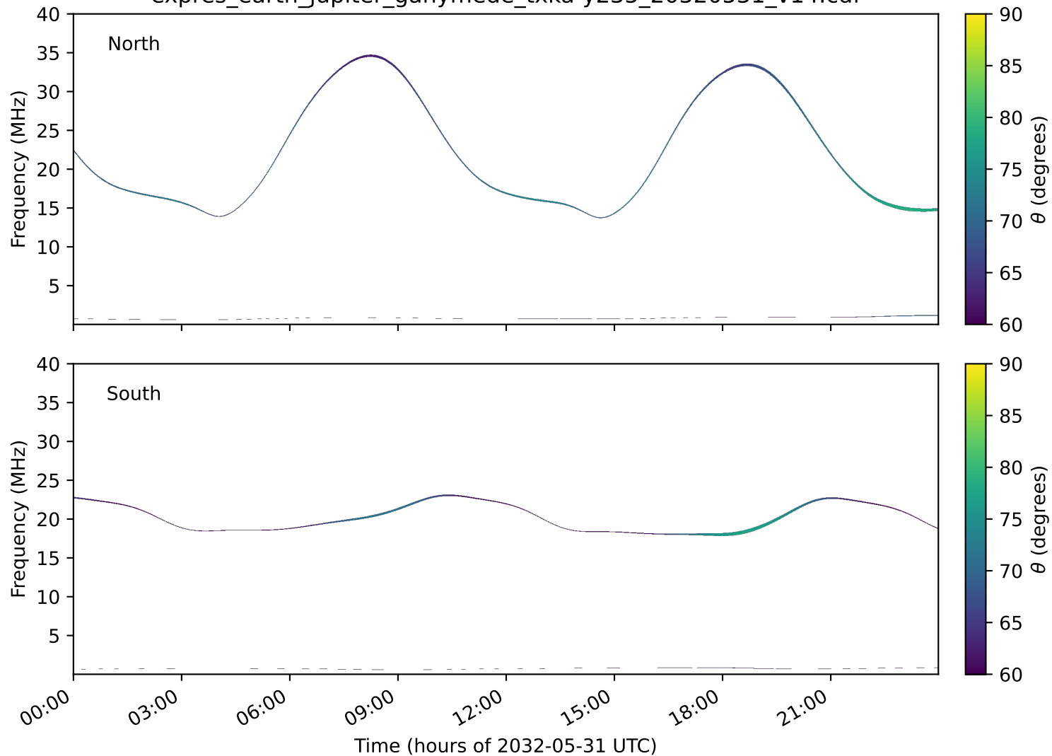
expres_earth_jupiter_ganymede_txka-y235_20320531_v14.cdf
