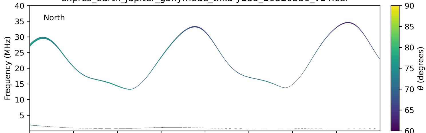
expres_earth_jupiter_ganymede_txka-y235_20320530_v14.cdf
