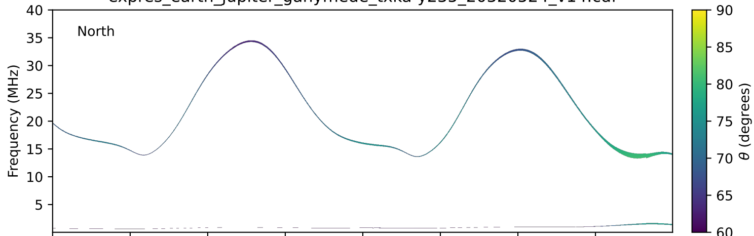
expres_earth_jupiter_ganymede_txka-y235_20320524_v14.cdf
