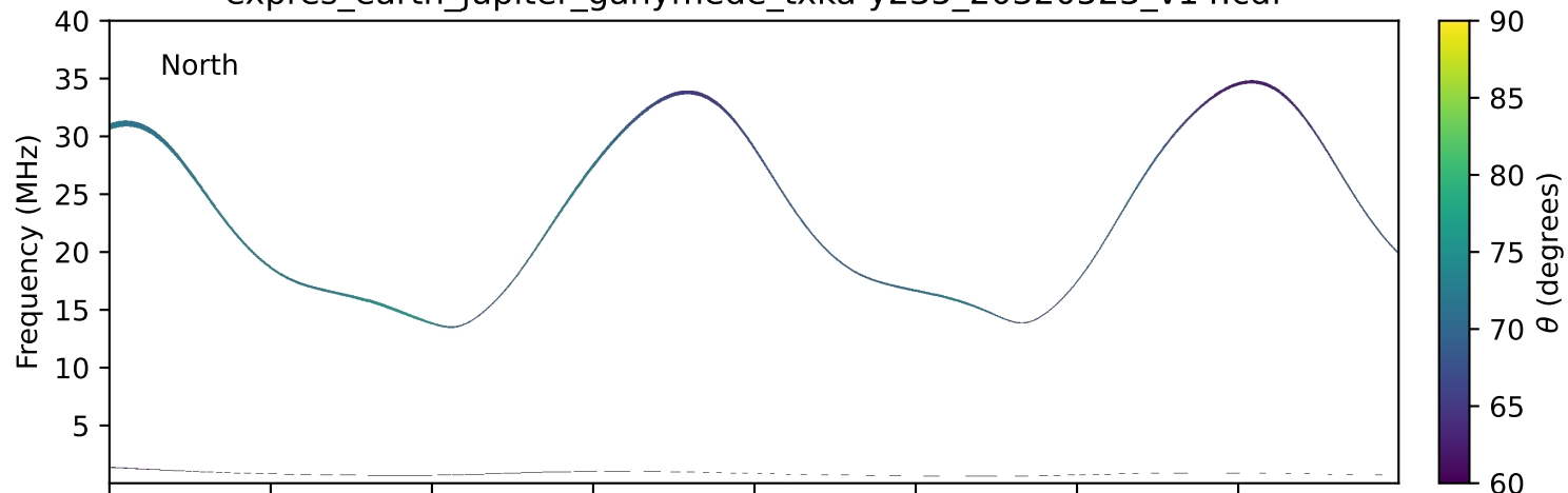
expres_earth_jupiter_ganymede_txka-y235_20320523_v14.cdf
