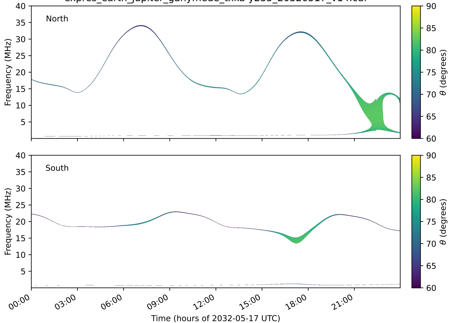
expres_earth_jupiter_ganymede_txka-y235_20320517_v14.cdf
