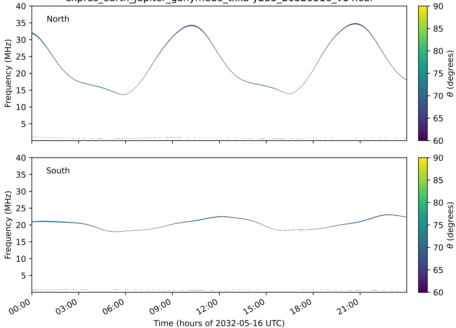
expres_earth_jupiter_ganymede_txka-y235_20320516_v14.cdf
