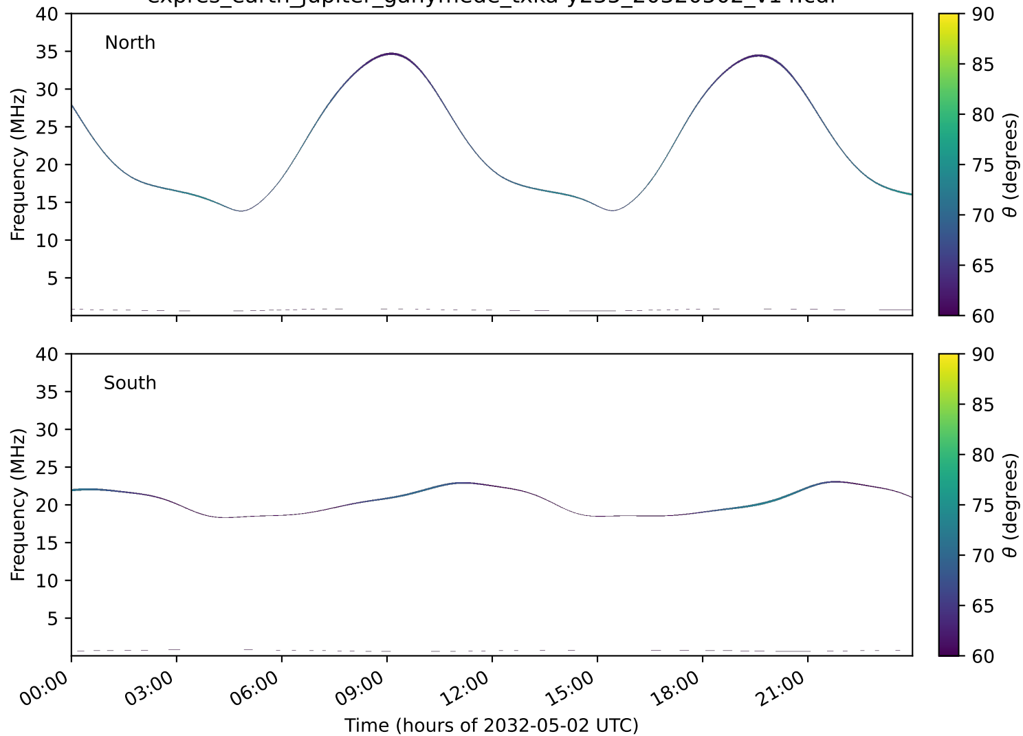
expres_earth_jupiter_ganymede_txka-y235_20320502_v14.cdf
