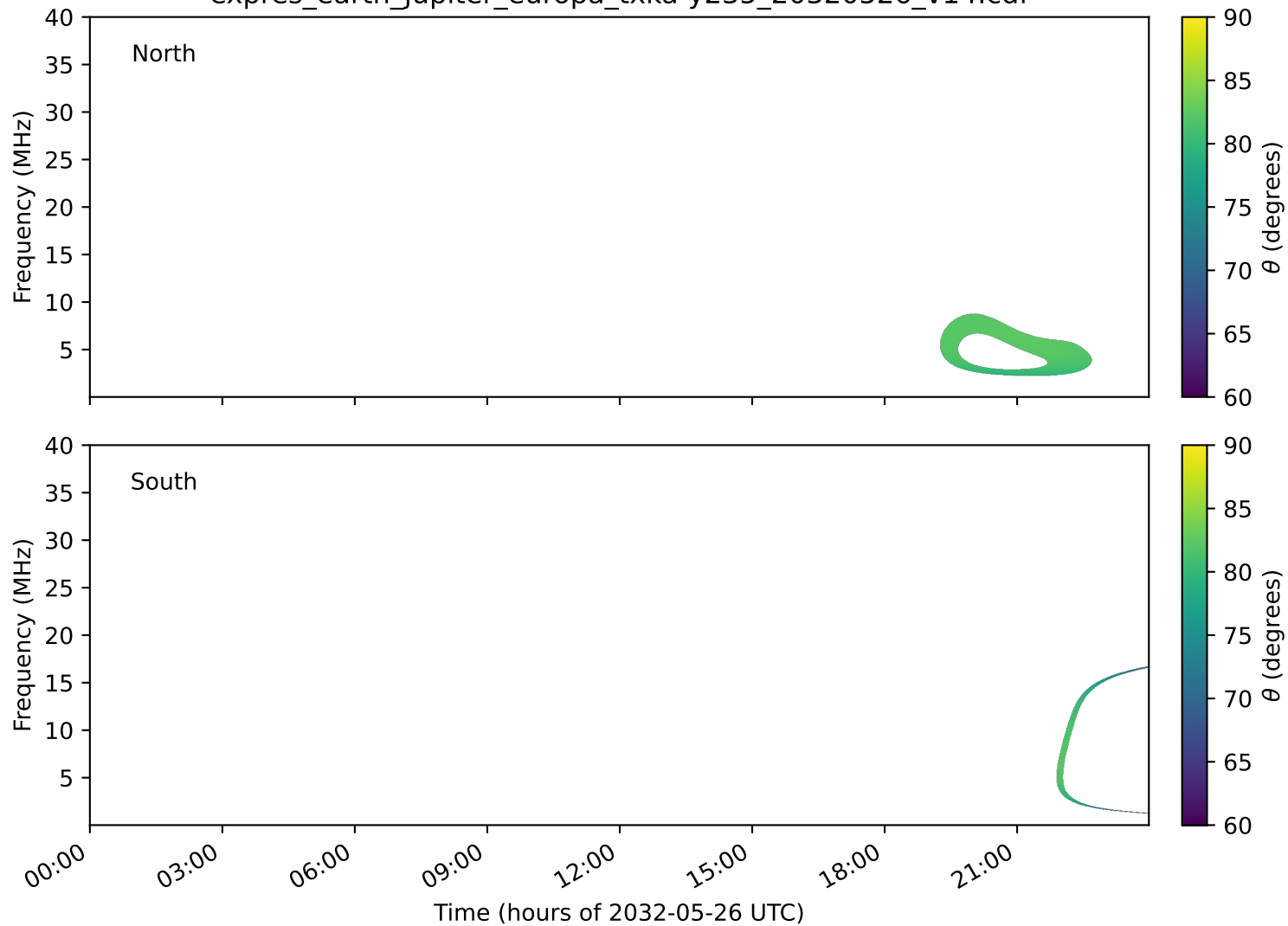
expres_earth_jupiter_europa_txka-y235_20320526_v14.cdf
