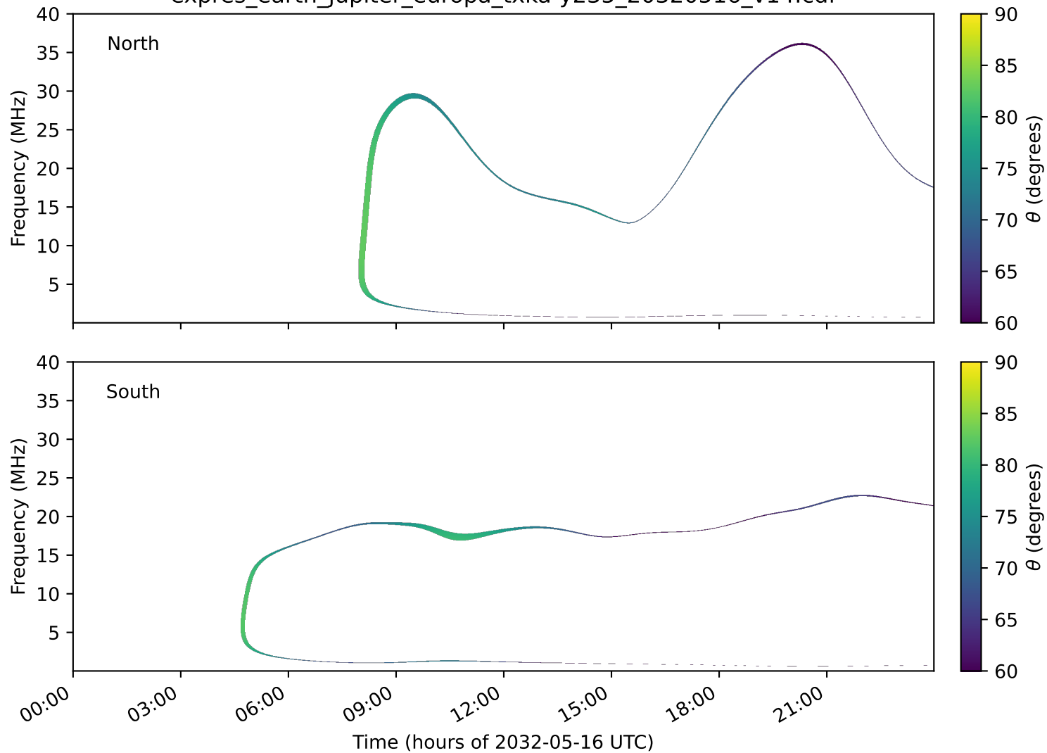
expres_earth_jupiter_europa_txka-y235_20320516_v14.cdf
