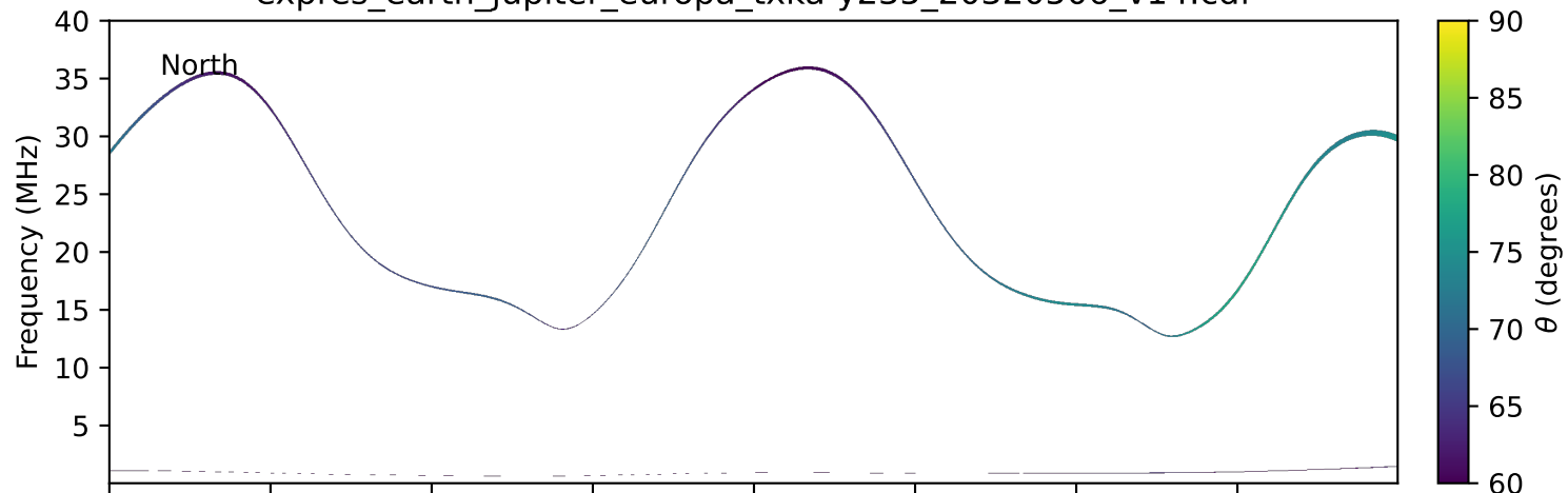
expres_earth_jupiter_europa_txka-y235_20320506_v14.cdf
