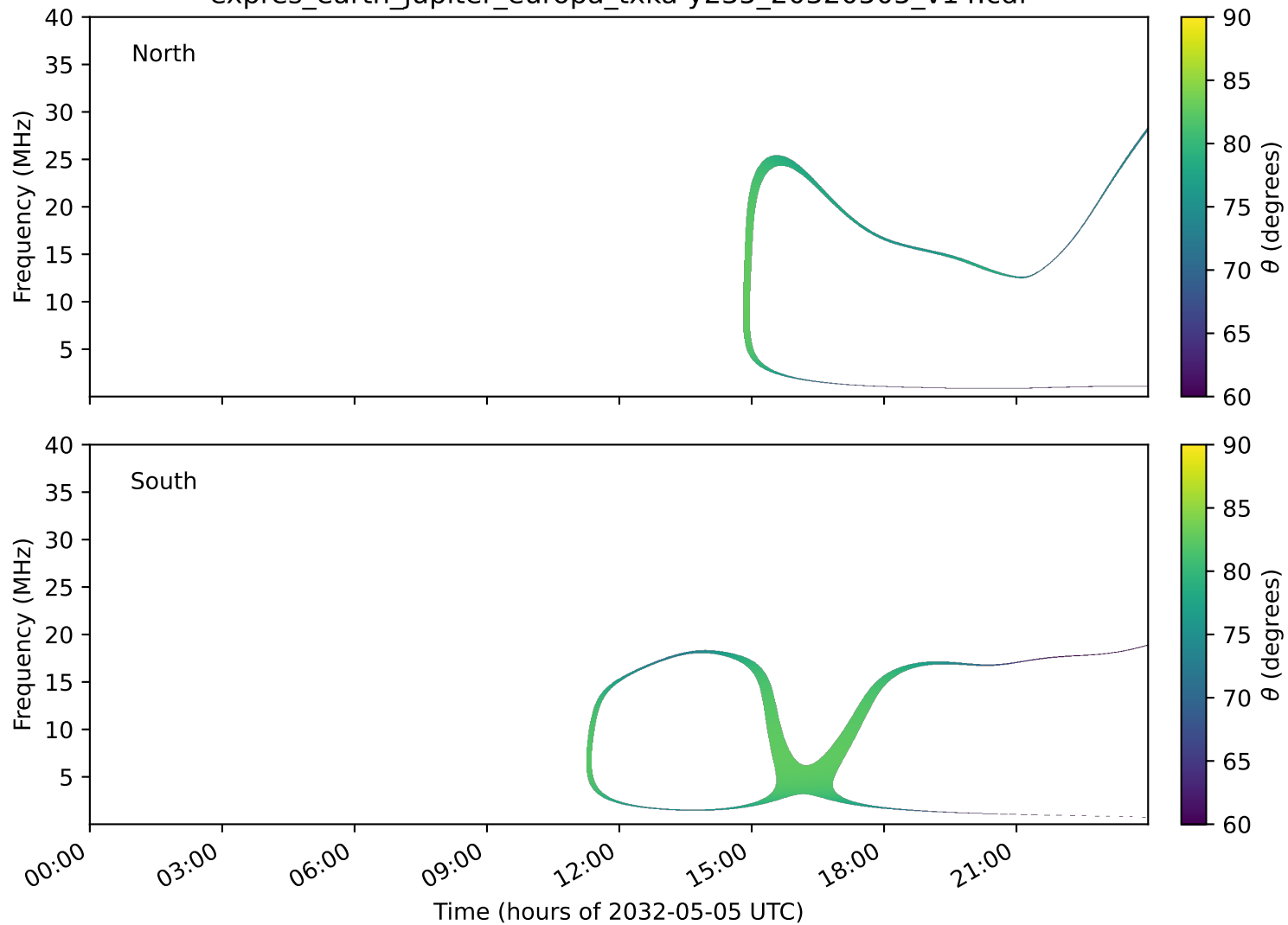
expres_earth_jupiter_europa_txka-y235_20320505_v14.cdf
