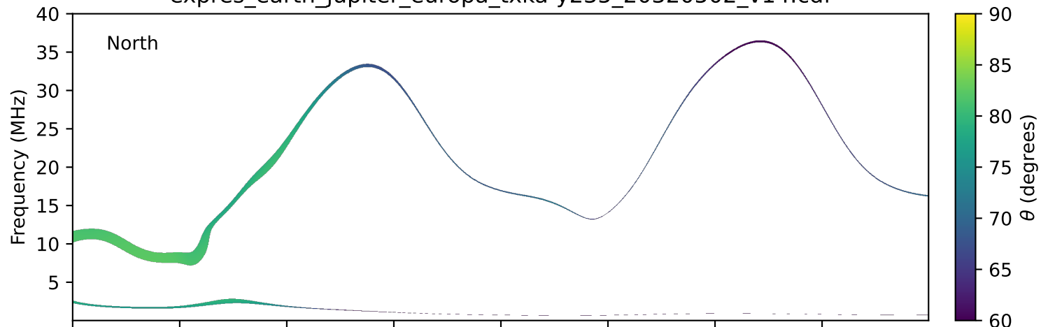
expres_earth_jupiter_europa_txka-y235_20320502_v14.cdf
