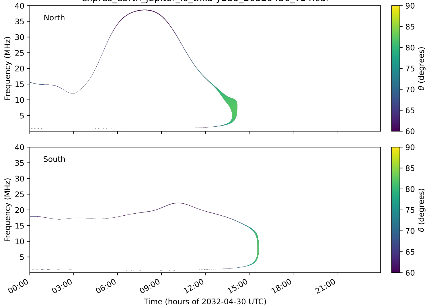
expres_earth_jupiter_io_txka-y235_20320430_v14.cdf
